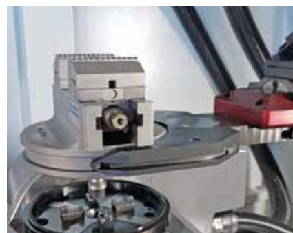
Mechanischer Zentrischspanner MZQ 170-60 PA, Erowa ITS 148 Mechanical centre-clamping vise MZQ 170-60 PA, Erowa ITS 148
